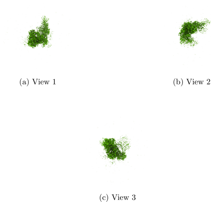
Figure 4: Isosurface at threshold=0.152000. Views generated by ChimeraX at a the following X, Y, Z angles: View 1 (0, -90, -90), View 2 (-90, 0, -90), View 3 (0, 0, 0).
