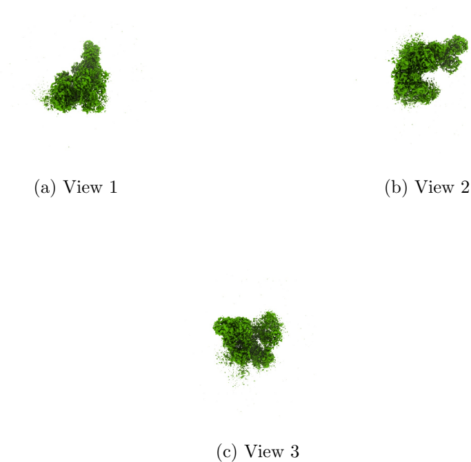
Figure 4: Isosurface at threshold=0.106000. Views generated by ChimeraX at a the following X, Y, Z angles: View 1 (0, -90, -90), View 2 (-90, 0, -90), View 3 (0, 0, 0).
