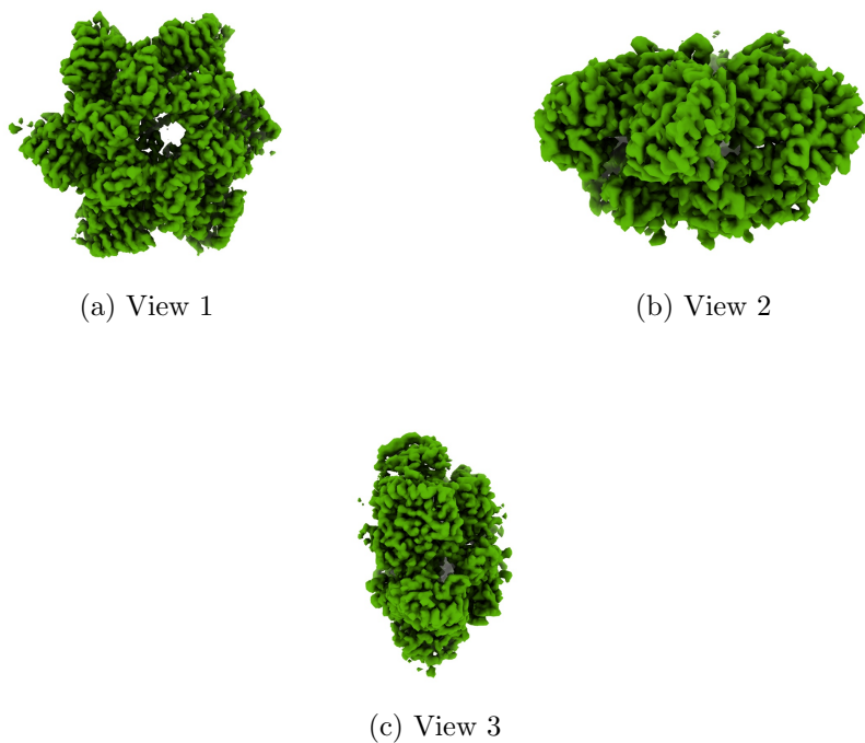
Figure 4: Isosurface at threshold=0.047800. Views generated by ChimeraX at a the following X, Y, Z angles: View 1 (0, -90, -90), View 2 (-90, 0, -90), View 3 (0, 0, 0).
