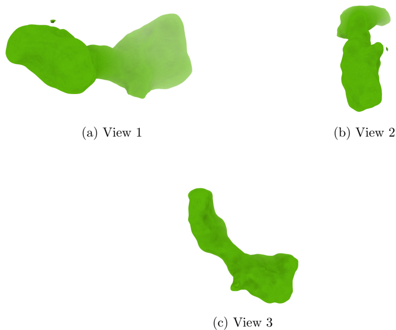
Figure 4: Isosurface at threshold=0.114000. Views generated by ChimeraX at a the following X, Y, Z angles: View 1 (0, -90, -90), View 2 (-90, 0, -90), View 3 (0, 0, 0).
