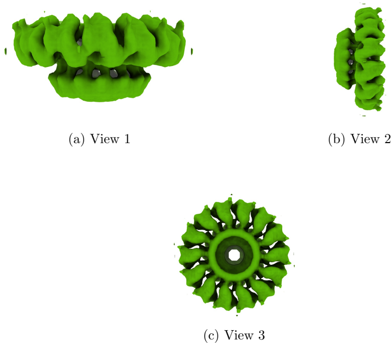
Figure 4: Isosurface at threshold=0.010800. Views generated by ChimeraX at a the following X, Y, Z angles: View 1 (0, -90, -90), View 2 (-90, 0, -90), View 3 (0, 0, 0).
