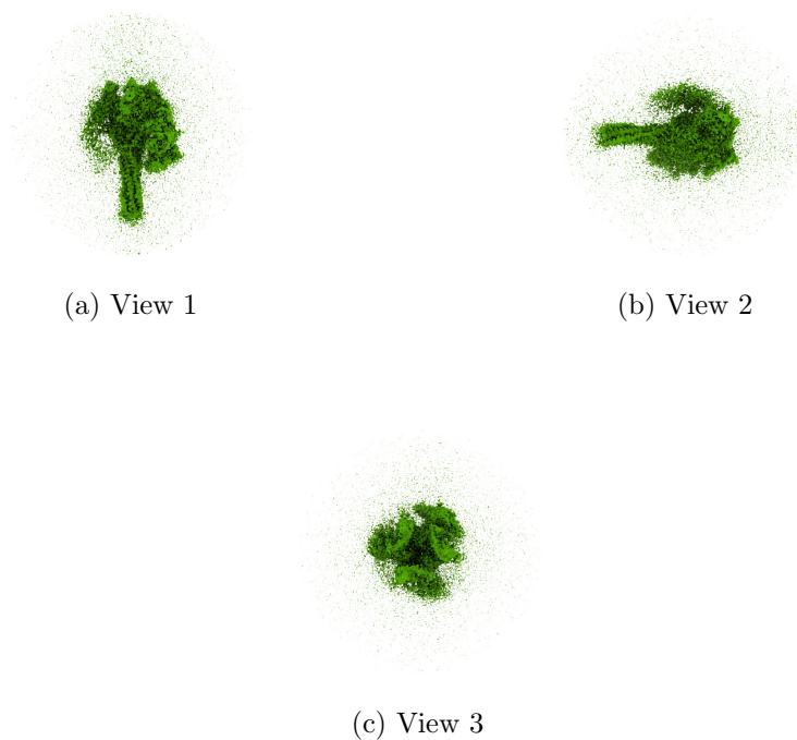
Figure 4: Isosurface at threshold=0.008100. Views generated by ChimeraX at a the following X, Y, Z angles: View 1 (0, -90, -90), View 2 (-90, 0, -90), View 3 (0, 0, 0).
