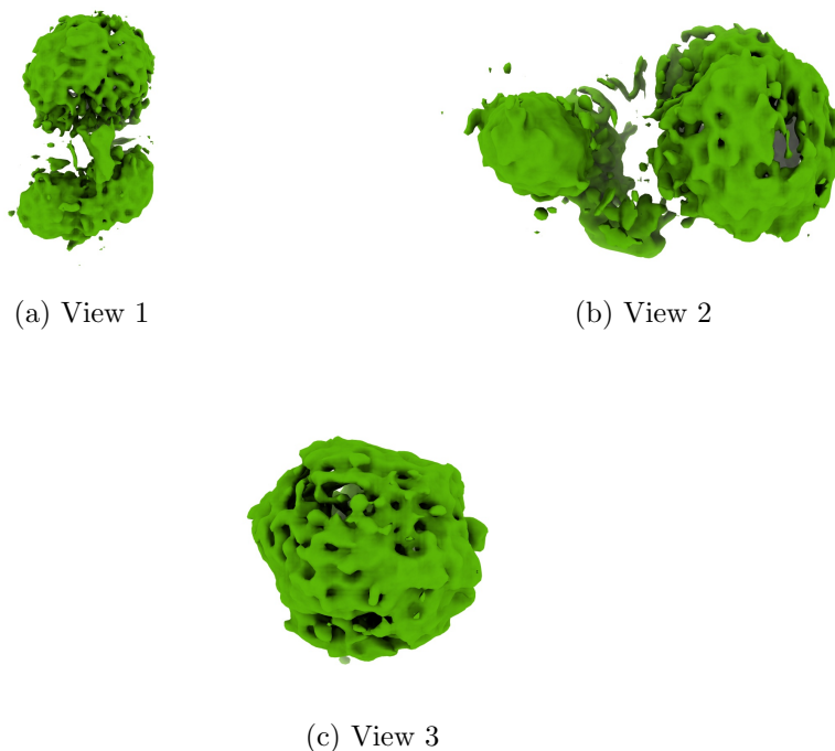
Figure 4: Isosurface at threshold=0.098900. Views generated by ChimeraX at a the following X, Y, Z angles: View 1 (0, -90, -90), View 2 (-90, 0, -90), View 3 (0, 0, 0).
