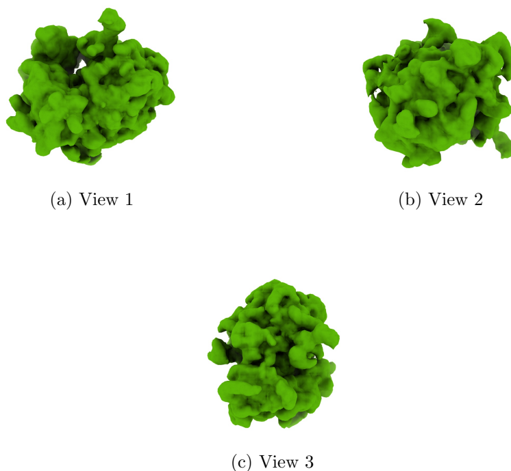
Figure 4: Isosurface at threshold=0.043300. Views generated by ChimeraX at a the following X, Y, Z angles: View 1 (0, -90, -90), View 2 (-90, 0, -90), View 3 (0, 0, 0).
