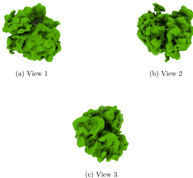
Figure 4: Isosurface at threshold=0.041500. Views generated by ChimeraX at a the following X, Y, Z angles: View 1 (0, -90, -90), View 2 (-90, 0, -90), View 3 (0, 0, 0).
