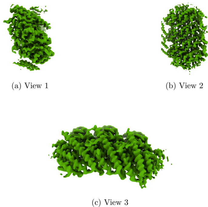
Figure 4: Isosurface at threshold=0.003810. Views generated by ChimeraX at a the following X, Y, Z angles: View 1 (0, -90, -90), View 2 (-90, 0, -90), View 3 (0, 0, 0).
