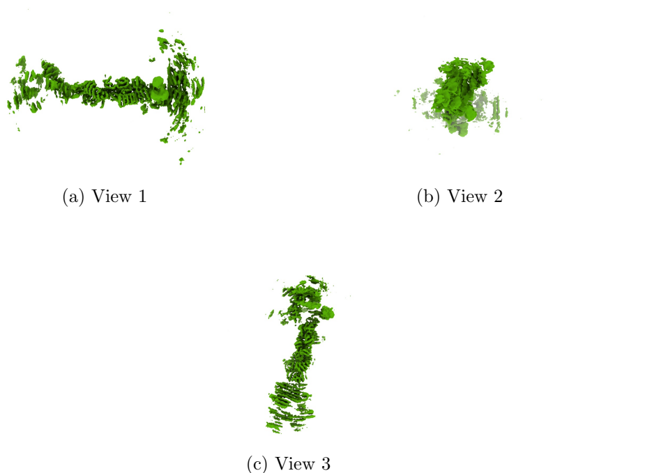
Figure 4: Isosurface at threshold=0.100000. Views generated by ChimeraX at a the following X, Y, Z angles: View 1 (0, -90, -90), View 2 (-90, 0, -90), View 3 (0, 0, 0).
