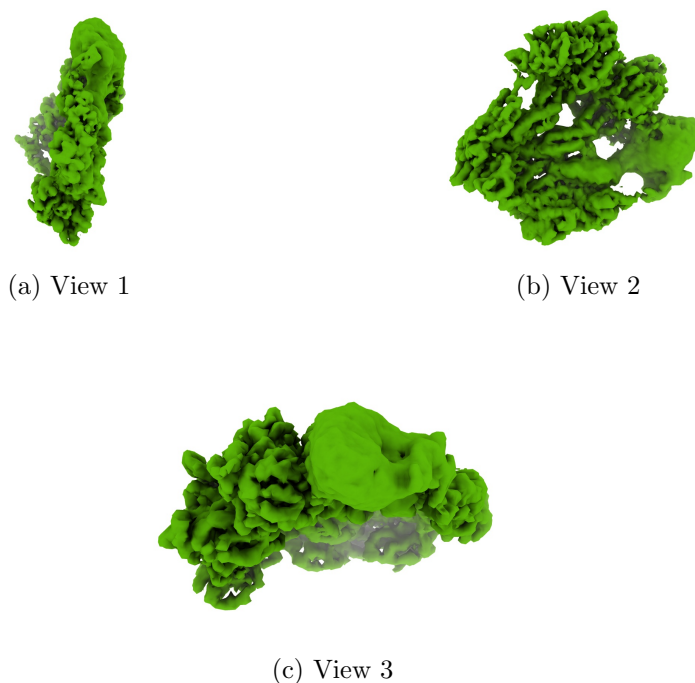
Figure 4: Isosurface at threshold=0.005500. Views generated by ChimeraX at a the following X, Y, Z angles: View 1 (0, -90, -90), View 2 (-90, 0, -90), View 3 (0, 0, 0).
