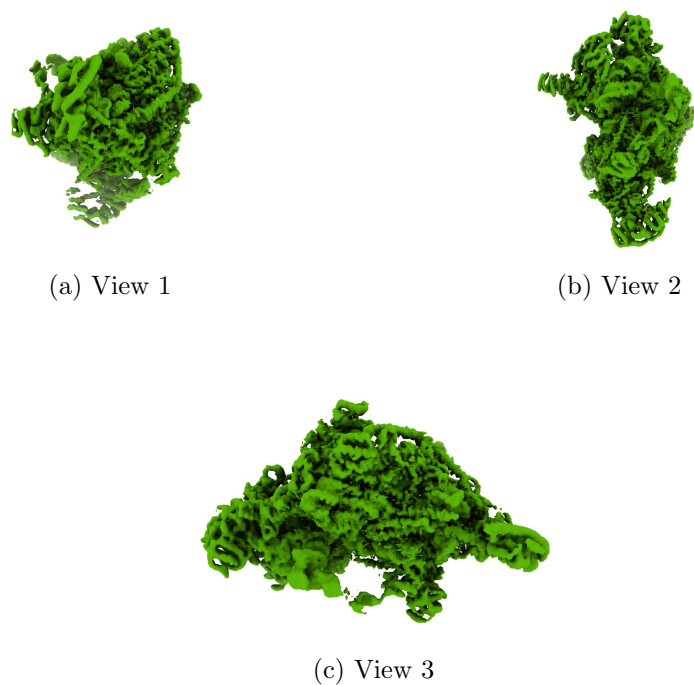
Figure 4: Isosurface at threshold=0.025600. Views generated by ChimeraX at a the following X, Y, Z angles: View 1 (0, -90, -90), View 2 (-90, 0, -90), View 3 (0, 0, 0).
