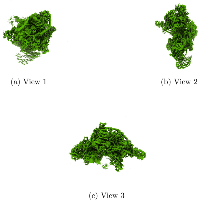
Figure 4: Isosurface at threshold=0.404000. Views generated by ChimeraX at a the following X, Y, Z angles: View 1 (0, -90, -90), View 2 (-90, 0, -90), View 3 (0, 0, 0).
