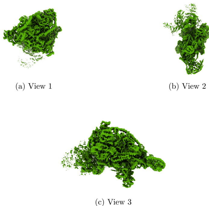
Figure 4: Isosurface at threshold=0.364000. Views generated by ChimeraX at a the following X, Y, Z angles: View 1 (0, -90, -90), View 2 (-90, 0, -90), View 3 (0, 0, 0).
