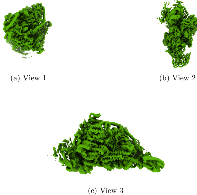
Figure 4: Isosurface at threshold=0.029400. Views generated by ChimeraX at a the following X, Y, Z angles: View 1 (0, -90, -90), View 2 (-90, 0, -90), View 3 (0, 0, 0).
