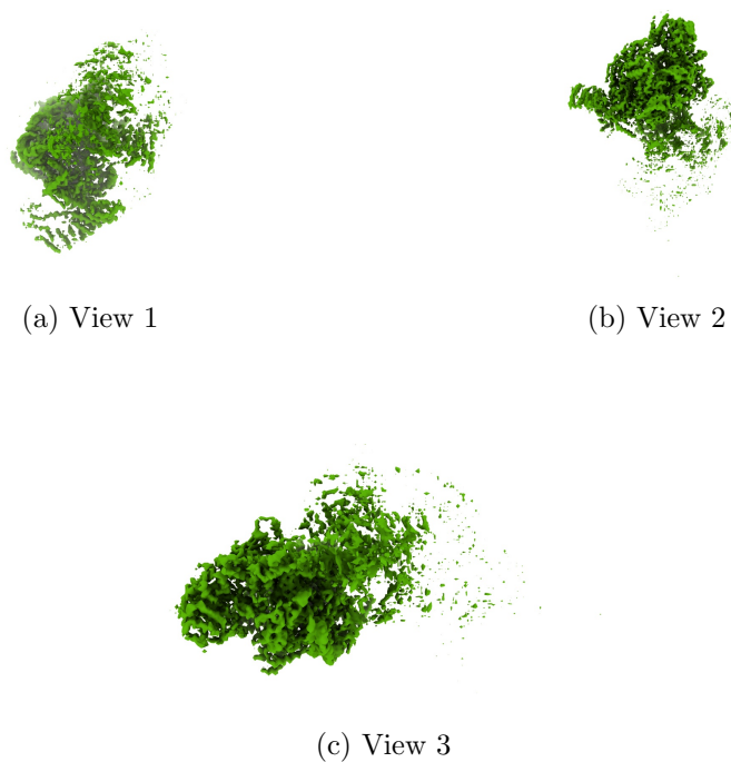
Figure 4: Isosurface at threshold=0.485000. Views generated by ChimeraX at a the following X, Y, Z angles: View 1 (0, -90, -90), View 2 (-90, 0, -90), View 3 (0, 0, 0).
