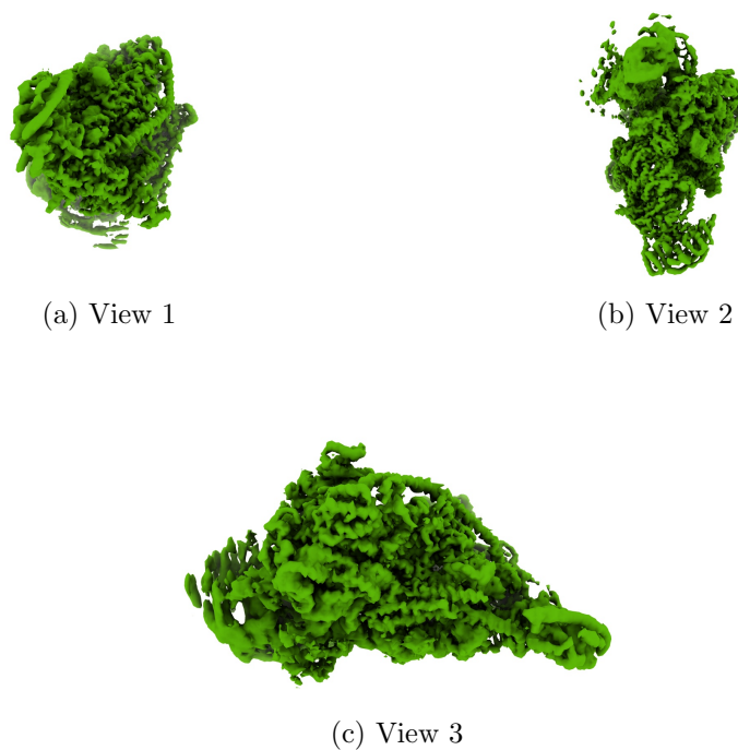
Figure 4: Isosurface at threshold=0.028100. Views generated by ChimeraX at a the following X, Y, Z angles: View 1 (0, -90, -90), View 2 (-90, 0, -90), View 3 (0, 0, 0).
