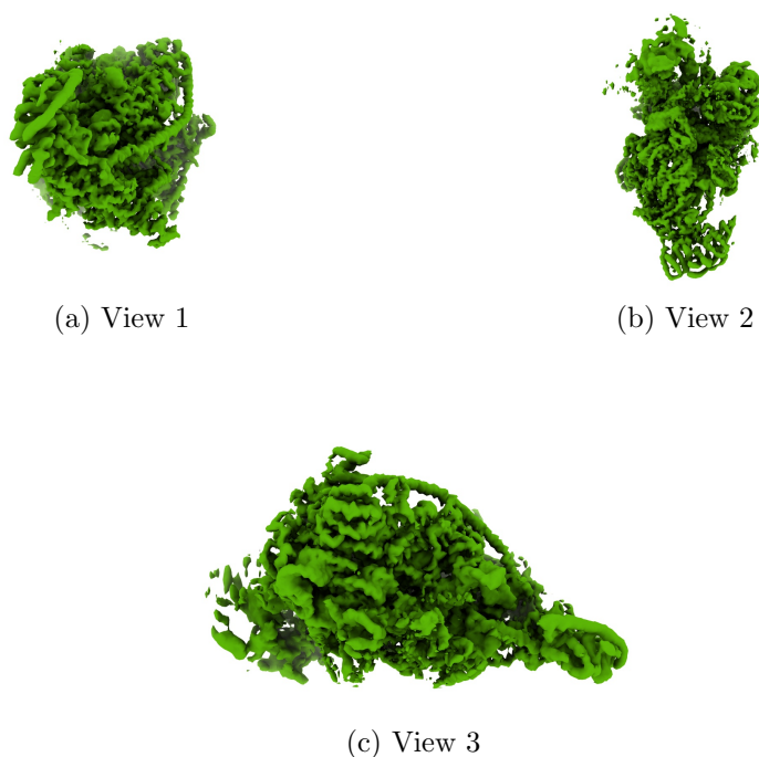
Figure 4: Isosurface at threshold=0.030200. Views generated by ChimeraX at a the following X, Y, Z angles: View 1 (0, -90, -90), View 2 (-90, 0, -90), View 3 (0, 0, 0).
