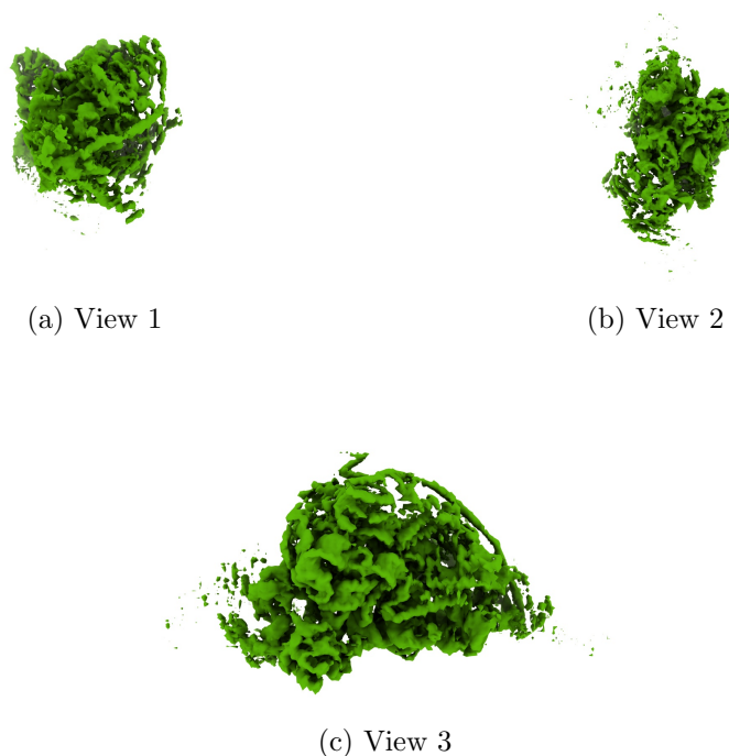
Figure 4: Isosurface at threshold=0.277000. Views generated by ChimeraX at a the following X, Y, Z angles: View 1 (0, -90, -90), View 2 (-90, 0, -90), View 3 (0, 0, 0).
