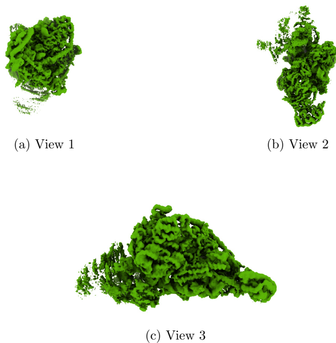
Figure 4: Isosurface at threshold=0.277000. Views generated by ChimeraX at a the following X, Y, Z angles: View 1 (0, -90, -90), View 2 (-90, 0, -90), View 3 (0, 0, 0).
