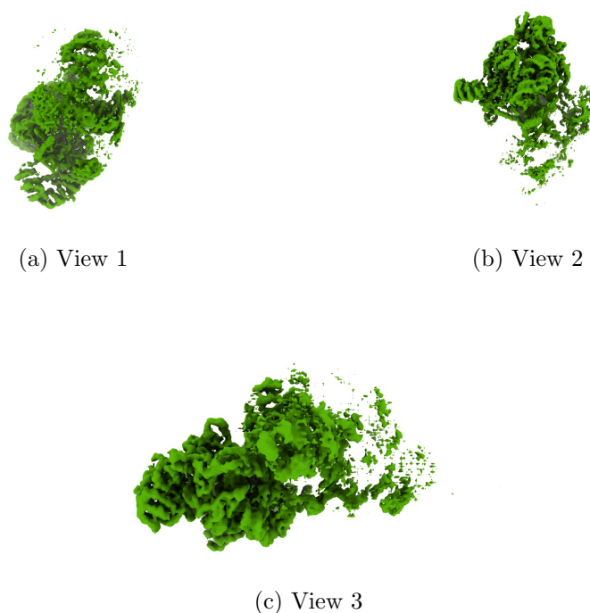
Figure 4: Isosurface at threshold=0.296000. Views generated by ChimeraX at a the following X, Y, Z angles: View 1 (0, -90, -90), View 2 (-90, 0, -90), View 3 (0, 0, 0).
