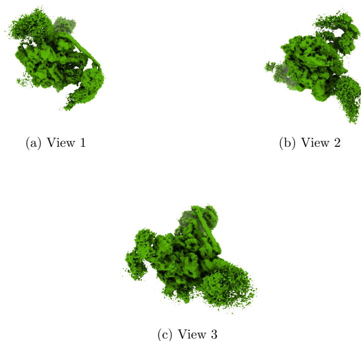
Figure 4: Isosurface at threshold=0.004430. Views generated by ChimeraX at a the following X, Y, Z angles: View 1 (0, -90, -90), View 2 (-90, 0, -90), View 3 (0, 0, 0).
