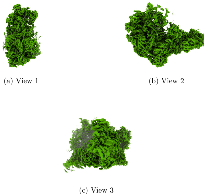
Figure 4: Isosurface at threshold=0.059900. Views generated by ChimeraX at a the following X, Y, Z angles: View 1 (0, -90, -90), View 2 (-90, 0, -90), View 3 (0, 0, 0).
