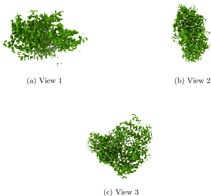
Figure 4: Isosurface at threshold=0.043800. Views generated by ChimeraX at a the following X, Y, Z angles: View 1 (0, -90, -90), View 2 (-90, 0, -90), View 3 (0, 0, 0).
