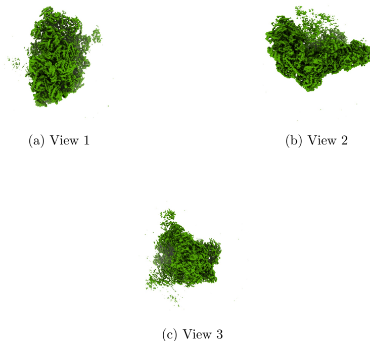
Figure 4: Isosurface at threshold=0.072600. Views generated by ChimeraX at a the following X, Y, Z angles: View 1 (0, -90, -90), View 2 (-90, 0, -90), View 3 (0, 0, 0).
