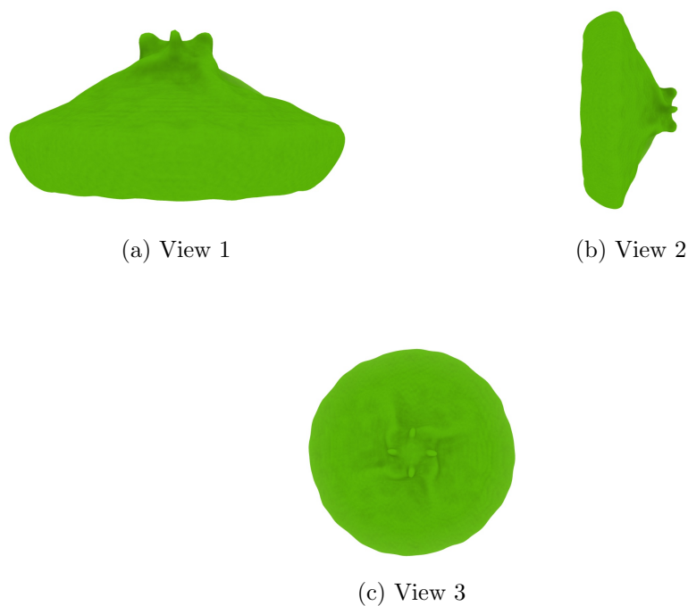
Figure 4: Isosurface at threshold=0.711000. Views generated by ChimeraX at a the following X, Y, Z angles: View 1 (0, -90, -90), View 2 (-90, 0, -90), View 3 (0, 0, 0).
