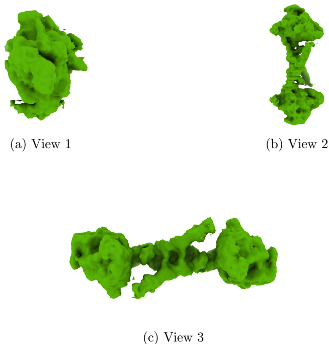
Figure 4: Isosurface at threshold=0.274000. Views generated by ChimeraX at a the following X, Y, Z angles: View 1 (0, -90, -90), View 2 (-90, 0, -90), View 3 (0, 0, 0).
