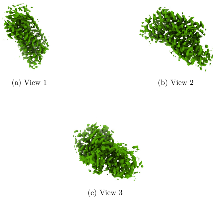
Figure 4: Isosurface at threshold=0.553000. Views generated by ChimeraX at a the following X, Y, Z angles: View 1 (0, -90, -90), View 2 (-90, 0, -90), View 3 (0, 0, 0).
