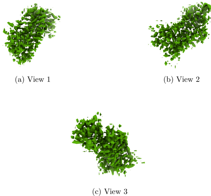
Figure 4: Isosurface at threshold=0.556000. Views generated by ChimeraX at a the following X, Y, Z angles: View 1 (0, -90, -90), View 2 (-90, 0, -90), View 3 (0, 0, 0).
