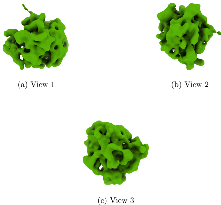
Figure 4: Isosurface at threshold=0.001410. Views generated by ChimeraX at a the following X, Y, Z angles: View 1 (0, -90, -90), View 2 (-90, 0, -90), View 3 (0, 0, 0).
