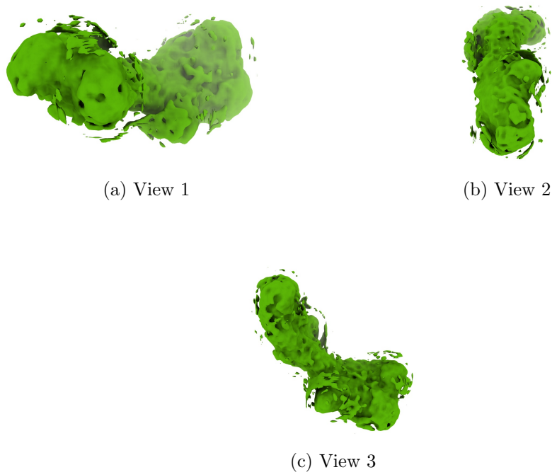
Figure 4: Isosurface at threshold=0.061800. Views generated by ChimeraX at a the following X, Y, Z angles: View 1 (0, -90, -90), View 2 (-90, 0, -90), View 3 (0, 0, 0).
