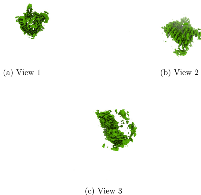
Figure 4: Isosurface at threshold=0.071700. Views generated by ChimeraX at a the following X, Y, Z angles: View 1 (0, -90, -90), View 2 (-90, 0, -90), View 3 (0, 0, 0).
