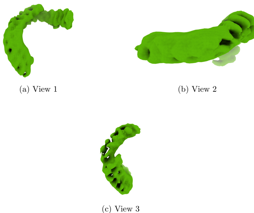
Figure 4: Isosurface at threshold=0.000900. Views generated by ChimeraX at a the following X, Y, Z angles: View 1 (0, -90, -90), View 2 (-90, 0, -90), View 3 (0, 0, 0).
