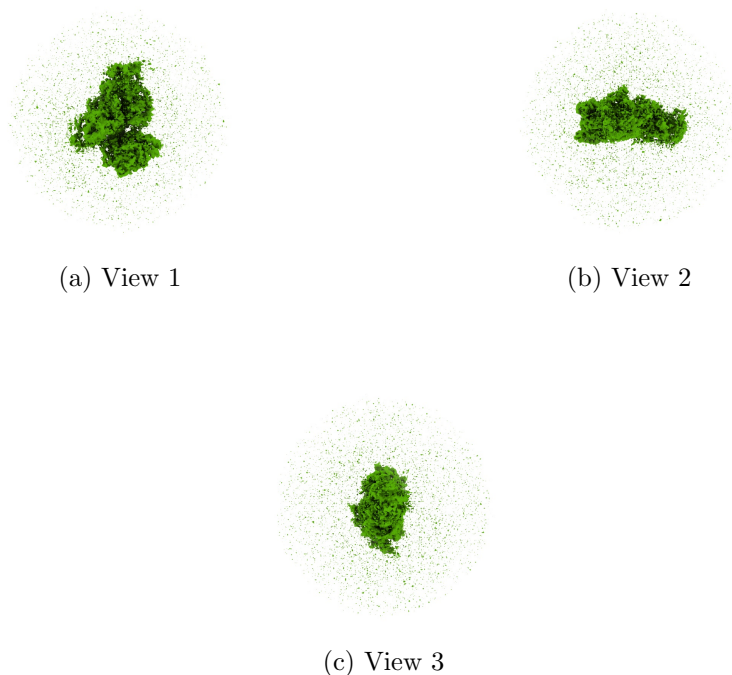
Figure 4: Isosurface at threshold=0.256000. Views generated by ChimeraX at a the following X, Y, Z angles: View 1 (0, -90, -90), View 2 (-90, 0, -90), View 3 (0, 0, 0).
