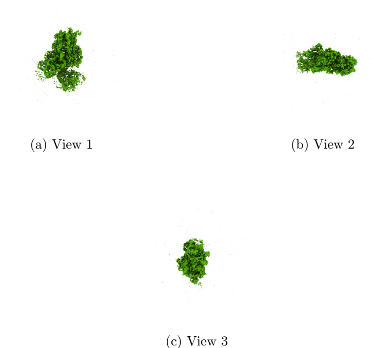
Figure 4: Isosurface at threshold=0.375000. Views generated by ChimeraX at a the following X, Y, Z angles: View 1 (0, -90, -90), View 2 (-90, 0, -90), View 3 (0, 0, 0).
