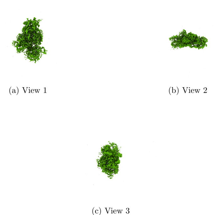
Figure 4: Isosurface at threshold=0.464000. Views generated by ChimeraX at a the following X, Y, Z angles: View 1 (0, -90, -90), View 2 (-90, 0, -90), View 3 (0, 0, 0).
