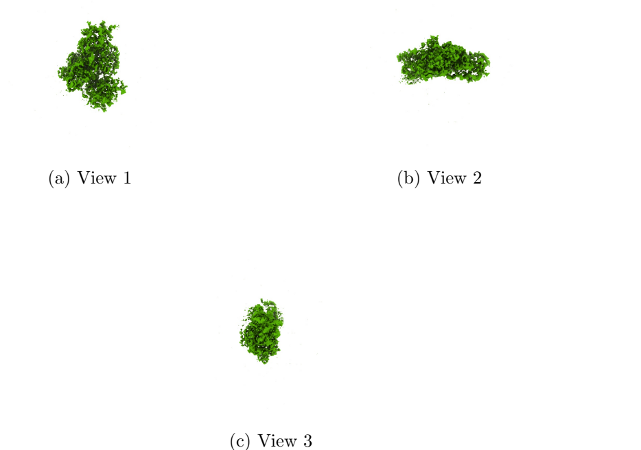
Figure 4: Isosurface at threshold=0.413000. Views generated by ChimeraX at a the following X, Y, Z angles: View 1 (0, -90, -90), View 2 (-90, 0, -90), View 3 (0, 0, 0).
