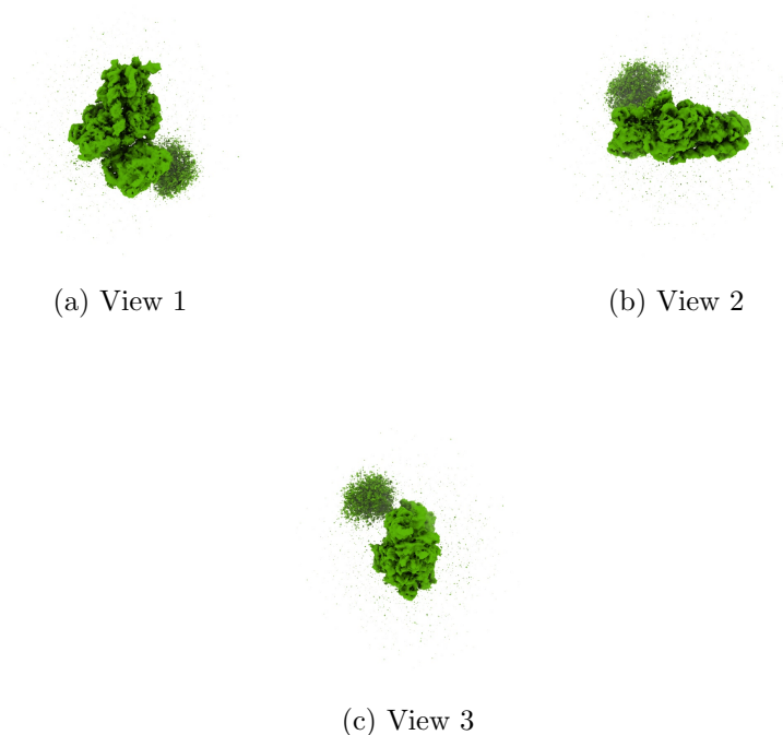
Figure 4: Isosurface at threshold=0.188000. Views generated by ChimeraX at a the following X, Y, Z angles: View 1 (0, -90, -90), View 2 (-90, 0, -90), View 3 (0, 0, 0).
