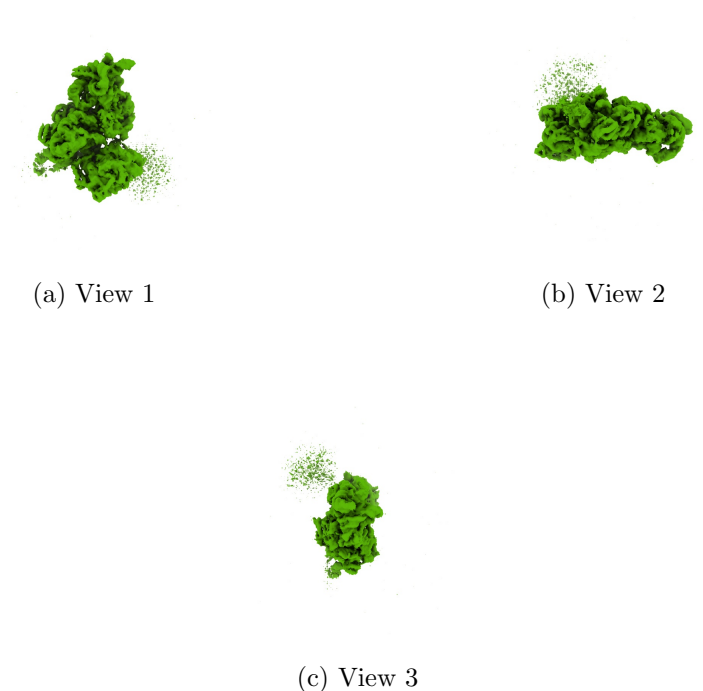
Figure 4: Isosurface at threshold=0.227000. Views generated by ChimeraX at a the following X, Y, Z angles: View 1 (0, -90, -90), View 2 (-90, 0, -90), View 3 (0, 0, 0).
