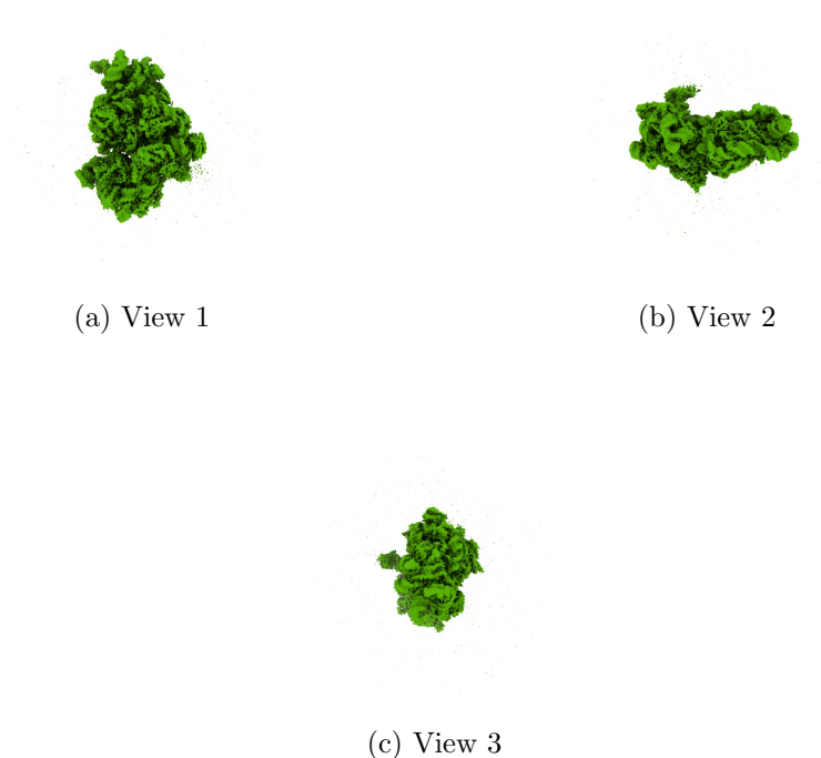
Figure 4: Isosurface at threshold=0.231000. Views generated by ChimeraX at a the following X, Y, Z angles: View 1 (0, -90, -90), View 2 (-90, 0, -90), View 3 (0, 0, 0).
