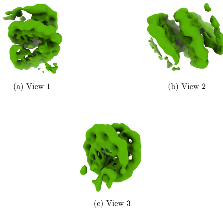
Figure 4: Isosurface at threshold=0.088700. Views generated by ChimeraX at a the following X, Y, Z angles: View 1 (0, -90, -90), View 2 (-90, 0, -90), View 3 (0, 0, 0).
