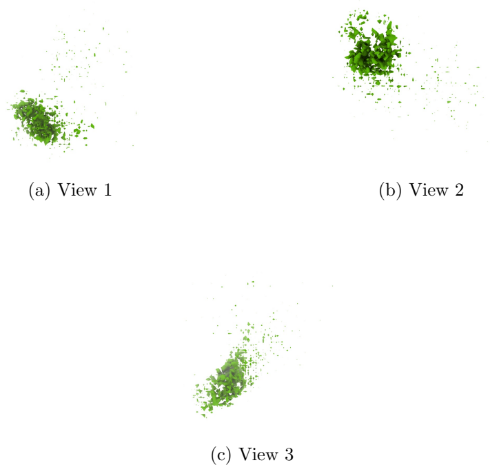
Figure 4: Isosurface at threshold=0.134000. Views generated by ChimeraX at a the following X, Y, Z angles: View 1 (0, -90, -90), View 2 (-90, 0, -90), View 3 (0, 0, 0).
