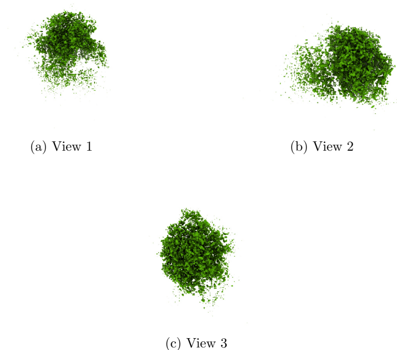
Figure 4: Isosurface at threshold=0.148000. Views generated by ChimeraX at a the following X, Y, Z angles: View 1 (0, -90, -90), View 2 (-90, 0, -90), View 3 (0, 0, 0).
