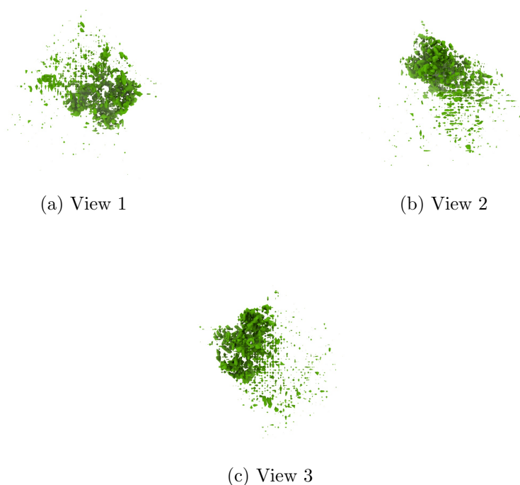
Figure 4: Isosurface at threshold=0.116000. Views generated by ChimeraX at a the following X, Y, Z angles: View 1 (0, -90, -90), View 2 (-90, 0, -90), View 3 (0, 0, 0).
