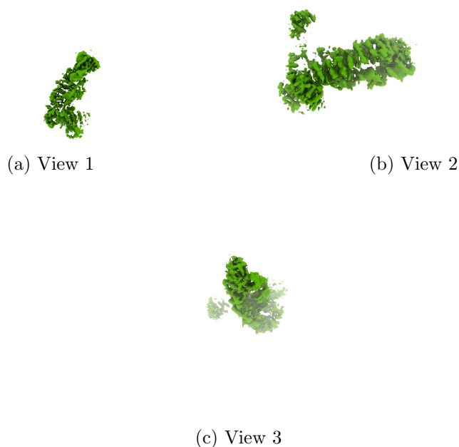
Figure 4: Isosurface at threshold=0.205000. Views generated by ChimeraX at a the following X, Y, Z angles: View 1 (0, -90, -90), View 2 (-90, 0, -90), View 3 (0, 0, 0).
