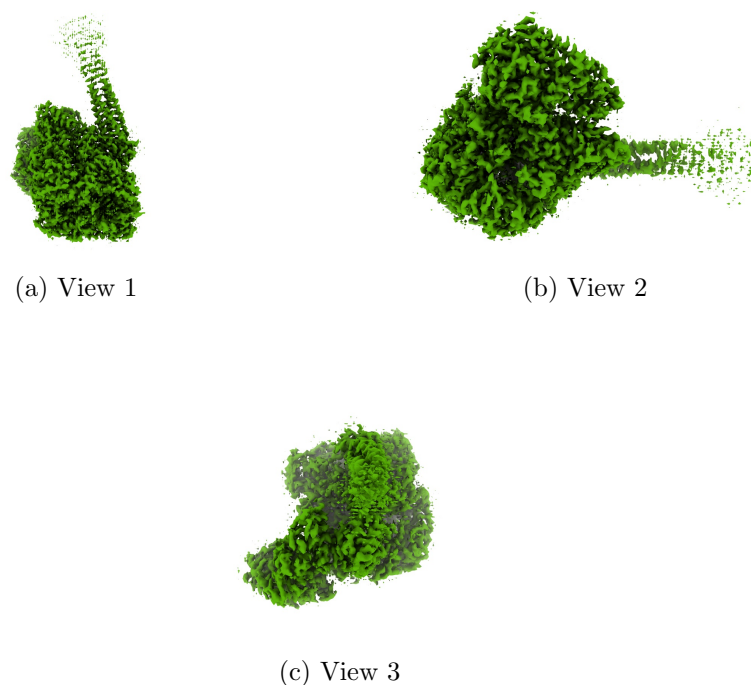
Figure 4: Isosurface at threshold=0.005460. Views generated by ChimeraX at a the following X, Y, Z angles: View 1 (0, -90, -90), View 2 (-90, 0, -90), View 3 (0, 0, 0).
