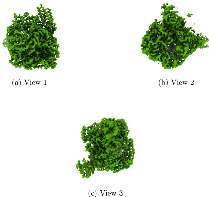
Figure 4: Isosurface at threshold=0.005670. Views generated by ChimeraX at a the following X, Y, Z angles: View 1 (0, -90, -90), View 2 (-90, 0, -90), View 3 (0, 0, 0).
