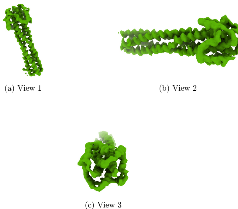
Figure 4: Isosurface at threshold=0.004530. Views generated by ChimeraX at a the following X, Y, Z angles: View 1 (0, -90, -90), View 2 (-90, 0, -90), View 3 (0, 0, 0).
