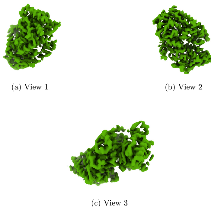
Figure 4: Isosurface at threshold=0.004340. Views generated by ChimeraX at a the following X, Y, Z angles: View 1 (0, -90, -90), View 2 (-90, 0, -90), View 3 (0, 0, 0).
